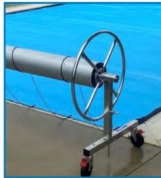
TITAN 150 150mm T-FRAME Stainless Steel, 3mm Wall 1.6mm Hand Wheel Square drive included as standard
